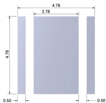
PCB Footprint
