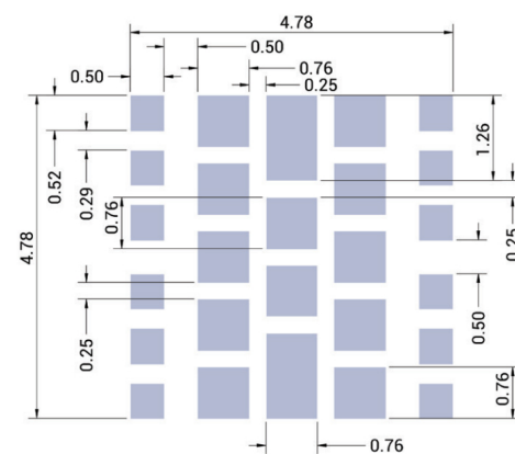
Stencil Opening
