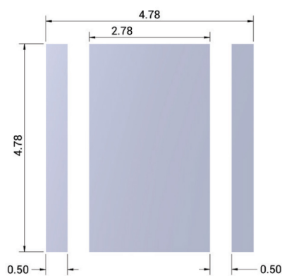
PCB Soldermask Opening
