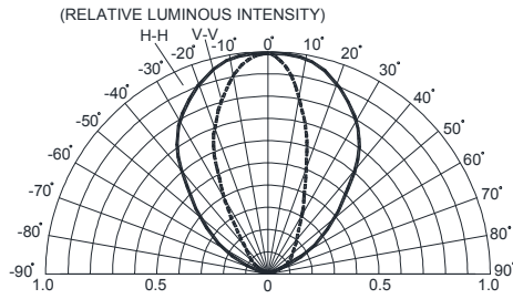
FIG.6b RED & BLUE&GREEN FAR FIELD PATTERN
