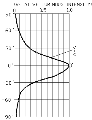
FIG.7 RED & BLUE&GREEN FAR FIELD PATTERN
