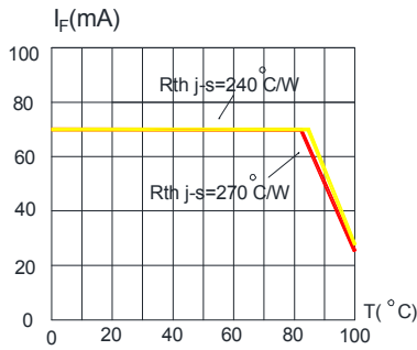
FIG.3 RED&AMBER MAXIMUM FORWARD DC CURRENT VS SOLDER TEMPERATURE ( T_{jmax}=110^{\circ}C )
