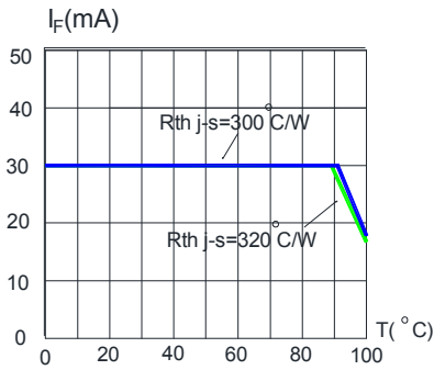
FIG.3 RED&AMBER MAXIMUM FORWARD DC CURRENT VS SOLDER TEMPERATURE ( T_{jmax}=110^{\circ}C )
