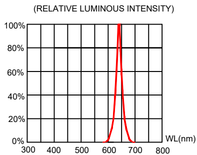
FIG.3 RELATIVE LUMINOUS INTENSITY VS. WAVELENGTH.
