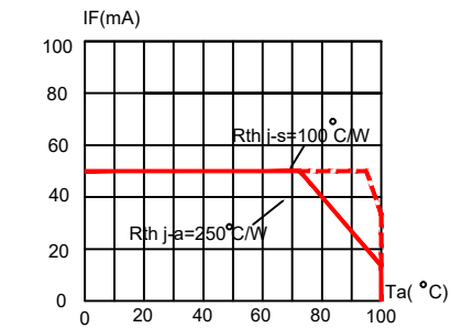
FIG.4 MAXIMUM FORWARD DC CURRENT VS AMBIENT TEMPERATURE ( T_{jmax}=110^{\circ}\text{C} )
