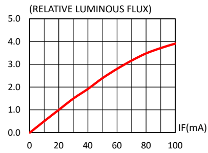
FIG.2 FORWARD LUMINOUS FLUX VS. FORWARD CURRENT
