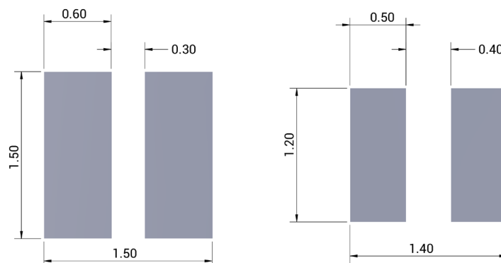
Recommended PCB Footprint
