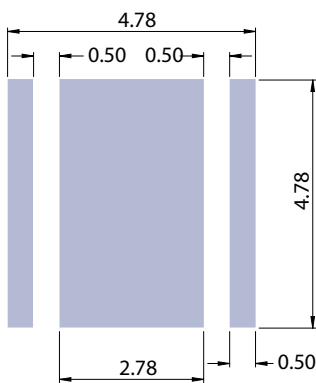
Recommended PCB Footprint
